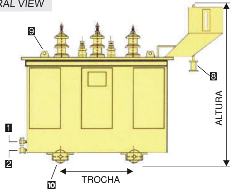
VISTA LATERAL LATERAL VIEW
